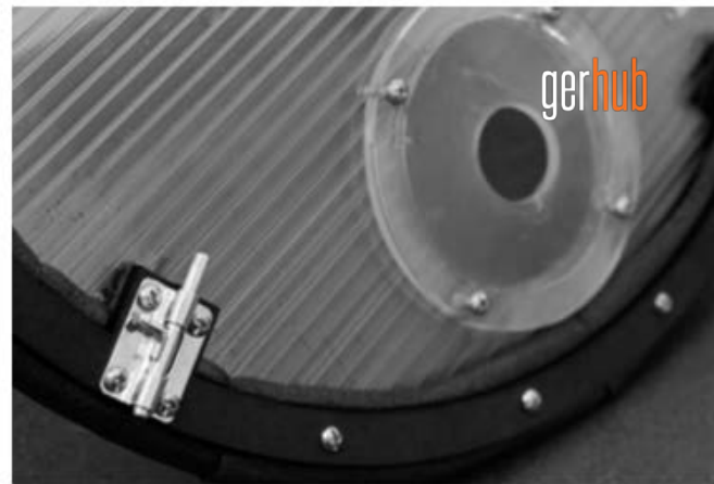
Figure 7. Locking mechanism and silicone chimney gasket
